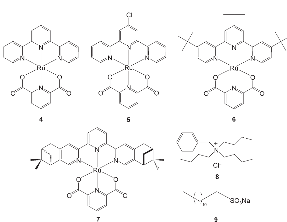
Scheme 2. Ruthenium catalysts and phase-transfer catalysts used for the synthesis of menadione ( 2 ).
