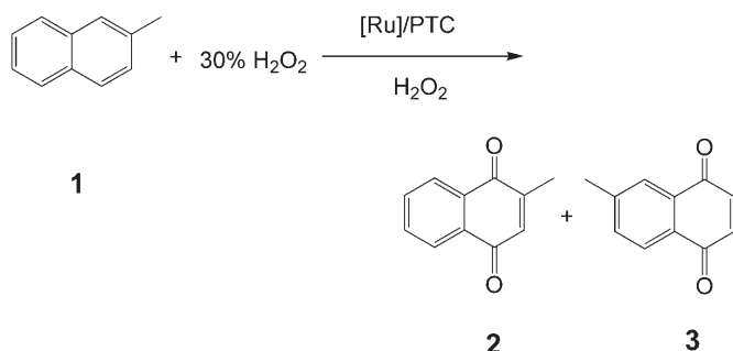
Scheme 1. Synthesis of 2-methyl-1,4-naphthoquinone (menadione).
